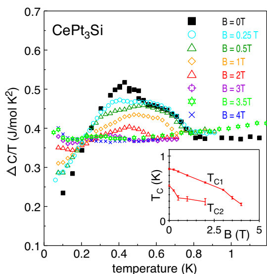
Figure 2. Temperature dependent \Delta C/T of CePt 3 Si (S2) in various magnetic fields (the AFM contribution was subtracted; see figure 1). The inset shows the magnetic field dependence of T_{C1} and T_{C2} .
